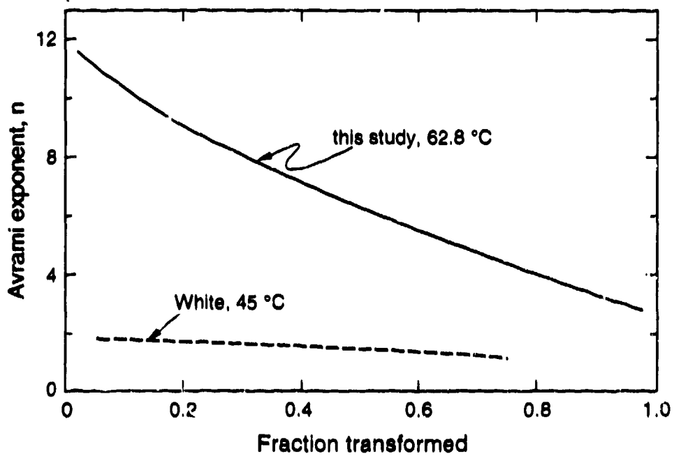
Figure 3. Avrami exponent versus fraction transformed for results of this study at 62.8 °C (see Figure 1) and White at 45 °C [3].
