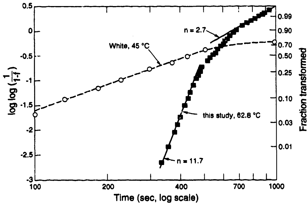
Figure 2. Johnson, Mehl, Avrami plot of \beta \rightarrow \alpha transformation measured at 62.8 °C by DSC in this study and at 45 °C by resistivity [3].
