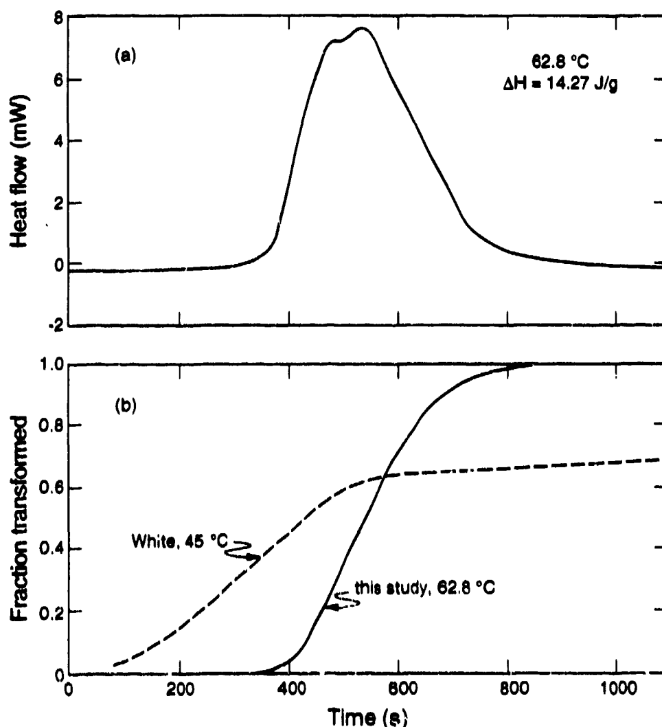
Figure 1. (a) Heat release peak for the \beta \rightarrow \alpha transformation at 62.8 °C. (b) Fraction transformed curve obtained by integrating heat flow peak in Figure 1a.
