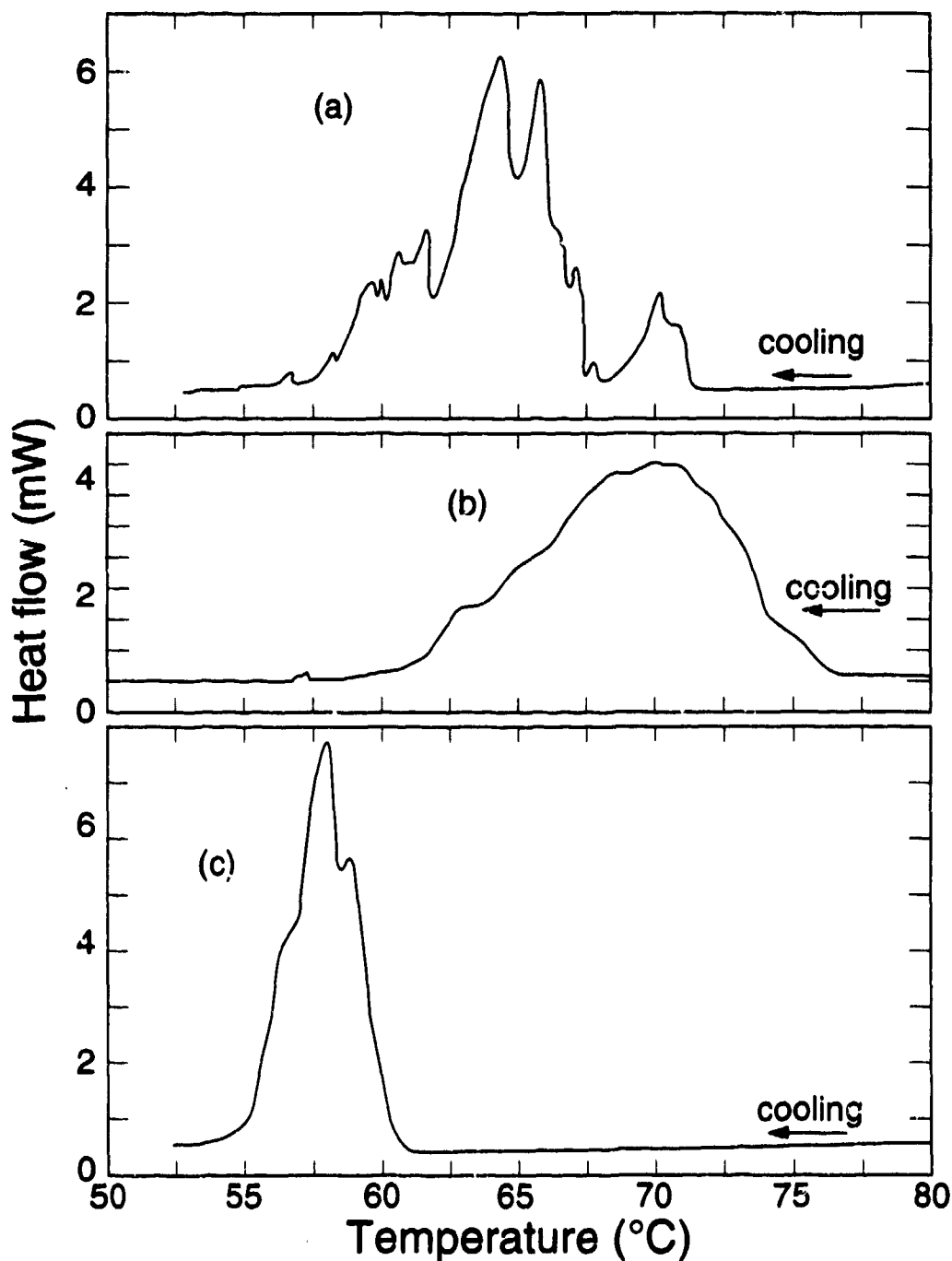
Figure 4. DSC measurements of the \beta \rightarrow \alpha transformation of a specimen consisting of ten pieces of plutonium. The ten pieces were simultaneously cooled through the transformation at roughly 1^\circ\text{C}/\text{min} . (a) First \beta \rightarrow \alpha transformation of as-received pieces. Measurements are during cooling immediately after the \alpha \rightarrow \beta reaction on heating to 150^\circ\text{C} . (b) Second \beta \rightarrow \alpha transformation of same samples upon cooling from 150^\circ\text{C} . (c) Fifteenth \beta \rightarrow \alpha transformation of same samples after 14 cycles of \alpha \rightarrow \beta \rightarrow \alpha transformation with intervening anneal for four days at room temperature.
